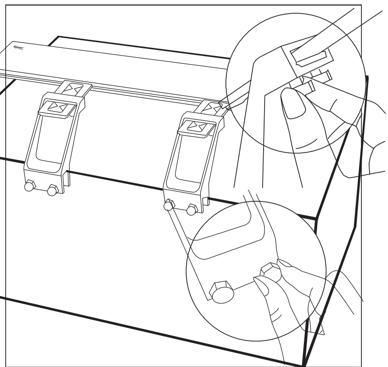
4.Put the light on the tank and tighten four screws.
